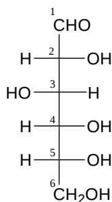
D-glucose (figure 1)
