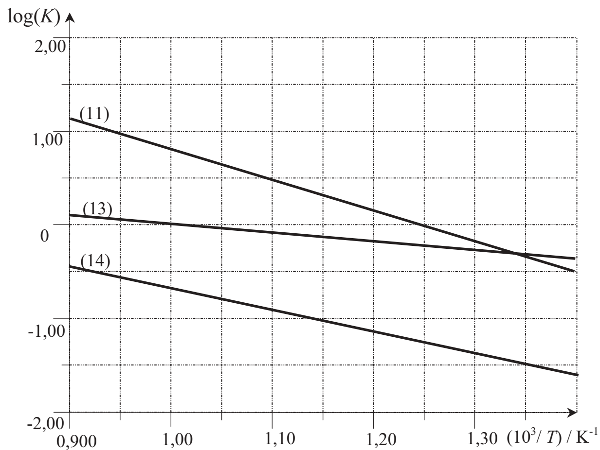
Figure 2 : \log(K) = f(1/T)
