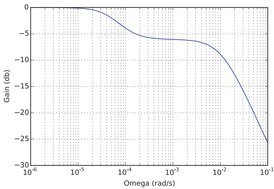
FIGURE 10 – Diagramme de Bode sans isolation
